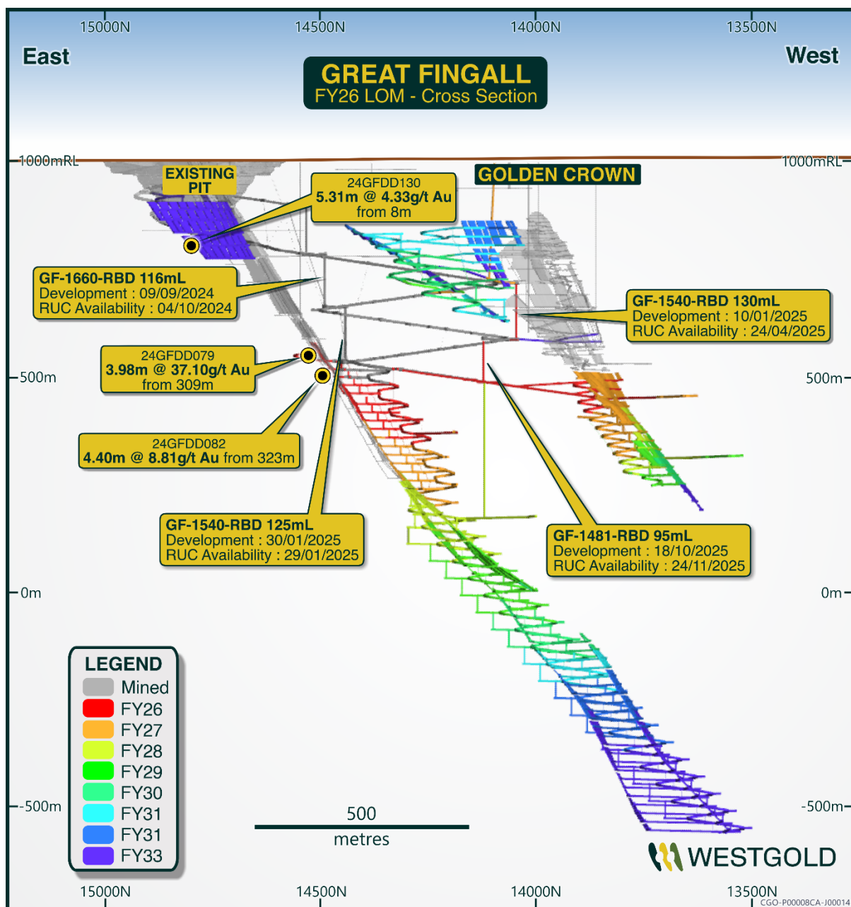
Figure 17 – Great Fingall Life of Mine Schematic FY26.
