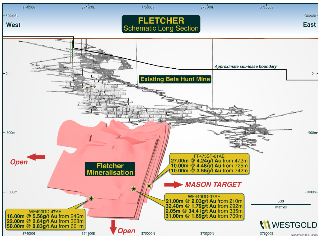
Figure 12 – Fletcher Zone Mineral Resource Schematic FY25.
