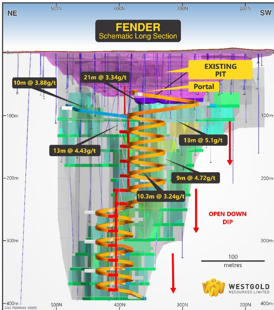
Figure 3: Fender Base Case Mine Design
