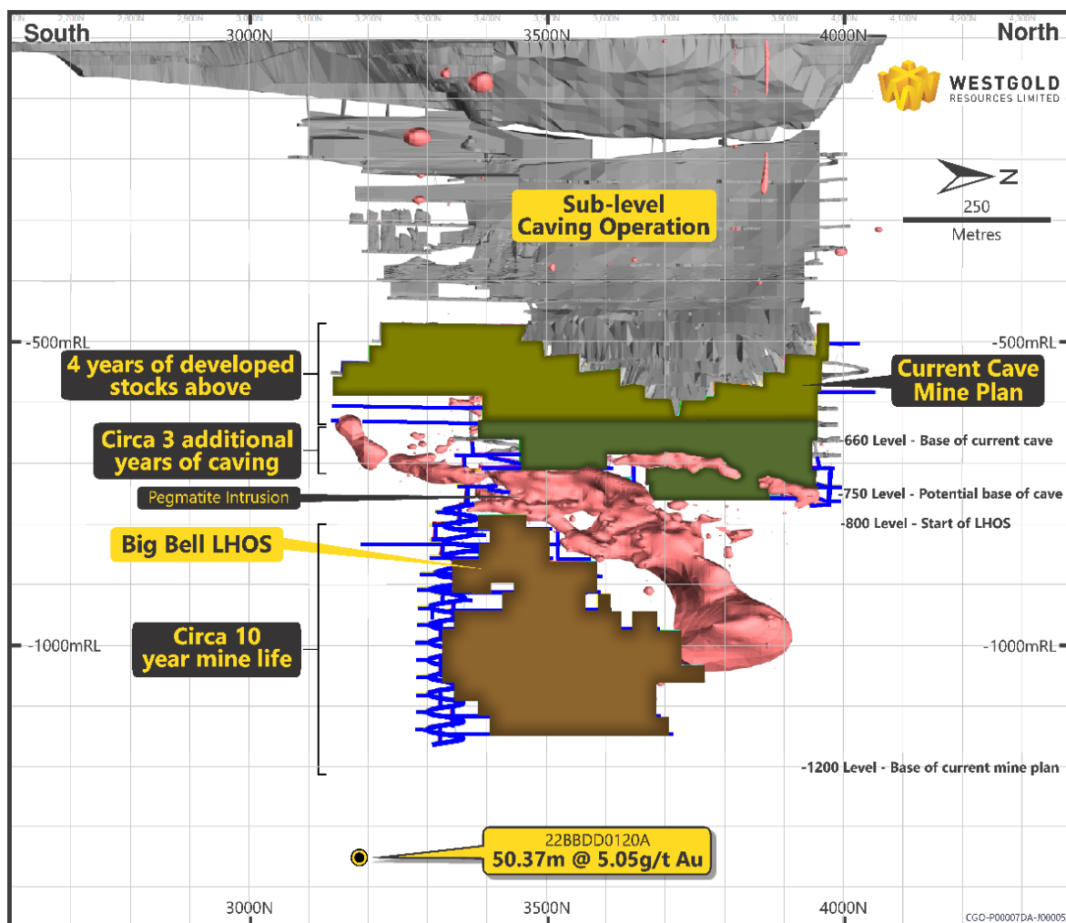
Figure 1: PFS Expansion Mine Layout with 22BBDD0120A Result
